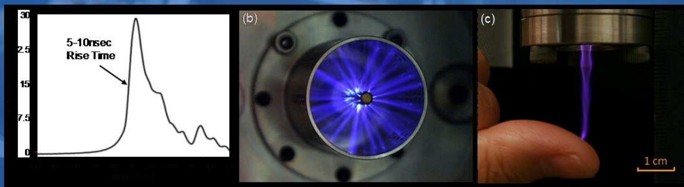
FIGURE 1. (A) TYPICAL OUTPUT CHARACTERISTICS OF NANOSECOND HIGH VOLTAGE PULSE GENERATOR. (B,C) PHOTOGRAPHS OF THE TRANSIENT PLASMA (HOT ELECTRON, LOW-TEMPERATURE PLASMA) FORMED BY THE HIGH VOLTAGE NANOSECOND PULSE APPROACH.
